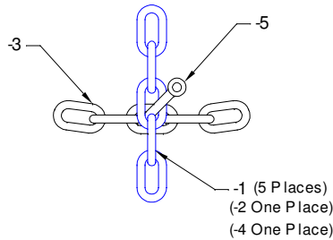
DETAIL - F Middle Connection
