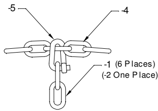
DETAIL - D Outer Connection
