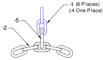
DETAIL - B Inner Connection
